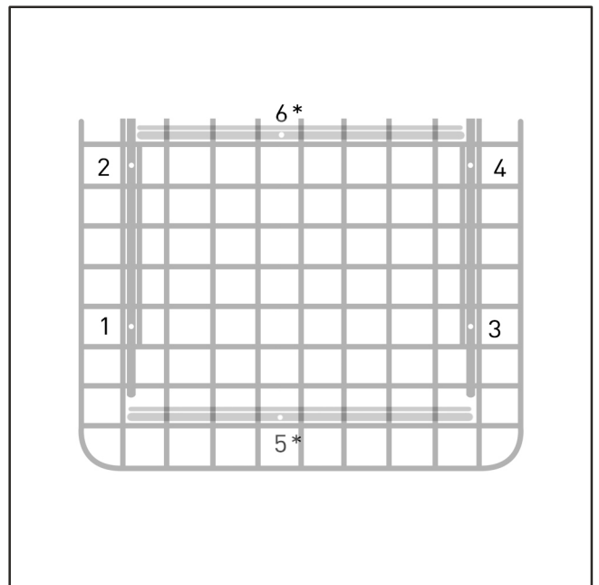
4. repeat step 3 four times. For the lounge chair* it should be repeated six times.
