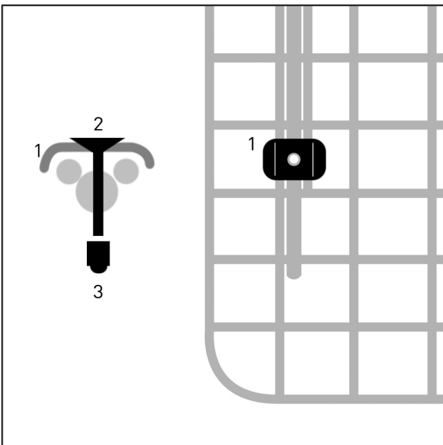
3. place the metal clip(1) onto the wires, over the hole. Insert the bolt(2) from the top and tighten the nut(3) at the underside.
